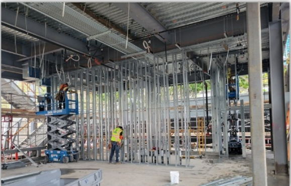
FUTURE STORAGE ROOM AND TELECOM WALL FRAMING ADJACENT TO KINDERGARTEN CLASSROOM A
